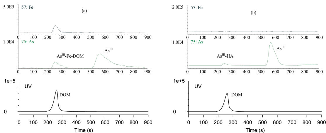
Figure 1. SEC-UV-ICP-MS chromatograms of \text{As}^{\text{III}} ( 50 \mu\text{g/L} ) complexation with (a) Fe-DOM (Fe=2.4 mg/L and DOC=14 mg/L) and (b) bare Aldrich HA (DOC=14 mg/L). Detection of Fe and As on ICP-MS and DOM peak on UV are shown in the chromatograms.
