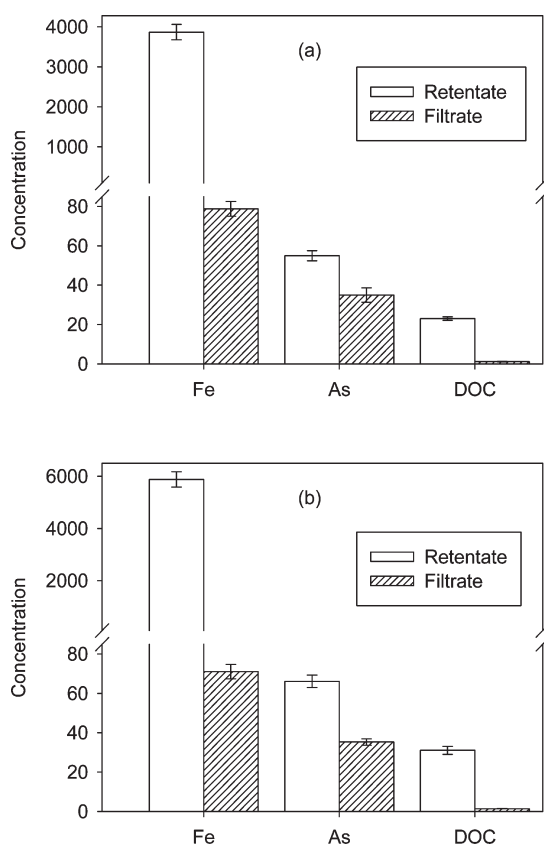
Figure 2. Distribution of Fe, As, and DOC present in \text{As}^{\text{III}} -Fe-DOM solutions (initial \text{As}^{\text{III}}=50 \mu\text{g/L} , \text{Fe}=2.4 \text{ mg/L} , and \text{DOC}=14 \text{ mg/L} ) between the retentates and filtrates after centrifugal filtration through (a) 1 kDa and (b) 3 kDa MWCO devices. Concentrations of Fe and As are in \mu\text{g/L} while DOC in \text{mg/L} .
