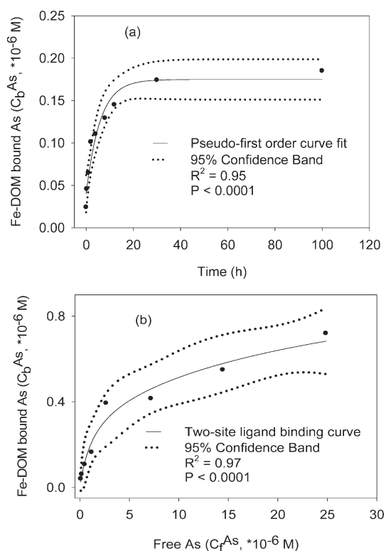
Figure 3. (a) Kinetic data of \text{As}^{\text{III}} (initial \text{As} = 100 \mu\text{g/L} ) complexation with Fe-DOM ( \text{Fe}=2.4 \text{ mg/L} and \text{DOC}=14 \text{ mg/L} ). (b) Calculation of K_s and B_{\text{max}} of \text{As}^{\text{III}} -Fe-DOM complexation through nonlinear regression using two-site ligand binding model.
