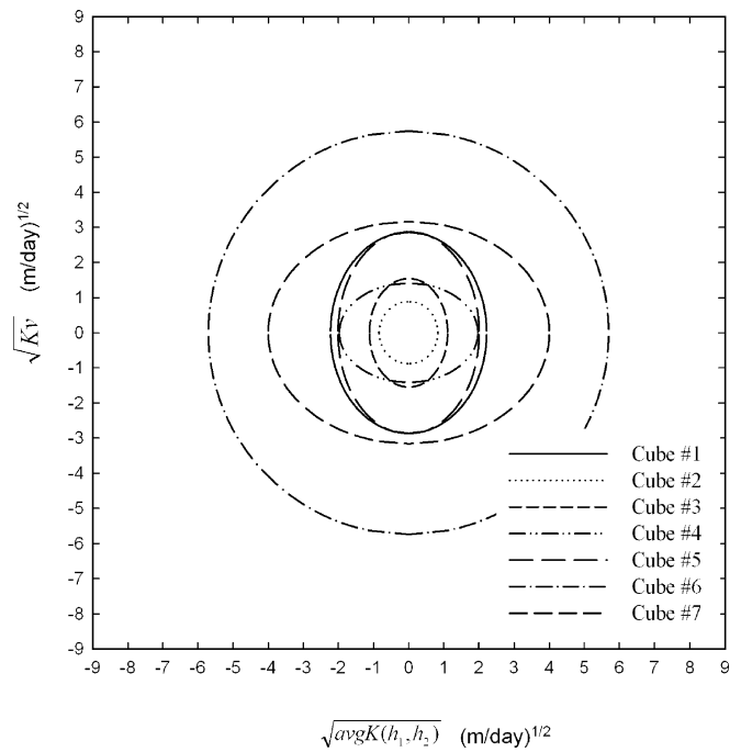
Fig. 9 Ellipse diagram showing anisotropy between vertical axis and horizontal axes of 0.2-m Key Largo Limestone cubes
