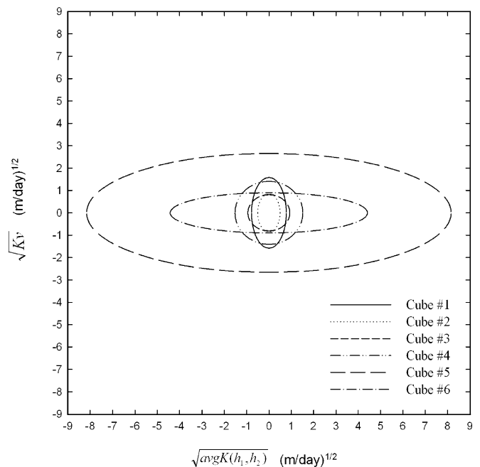
Fig. 10 Ellipse diagram showing anisotropy between vertical axis and horizontal axes of 0.3-m Key Largo Limestone cubes
