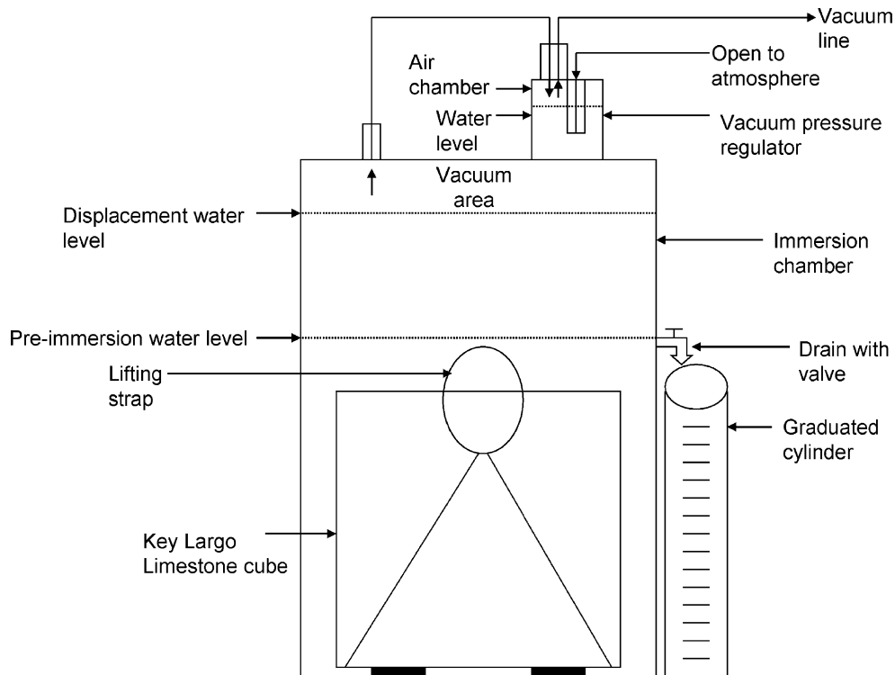
Fig. 3 Plexiglass chamber used to measure effective porosity. Vacuum regulator is on top of the chamber
