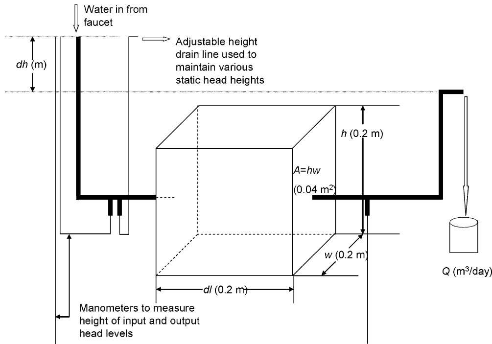
Fig. 4 Permeameter used to determine hydraulic conductivity values for each axis of Key Largo Limestone cubes. Water entered and left the cube through equalizing chambers
