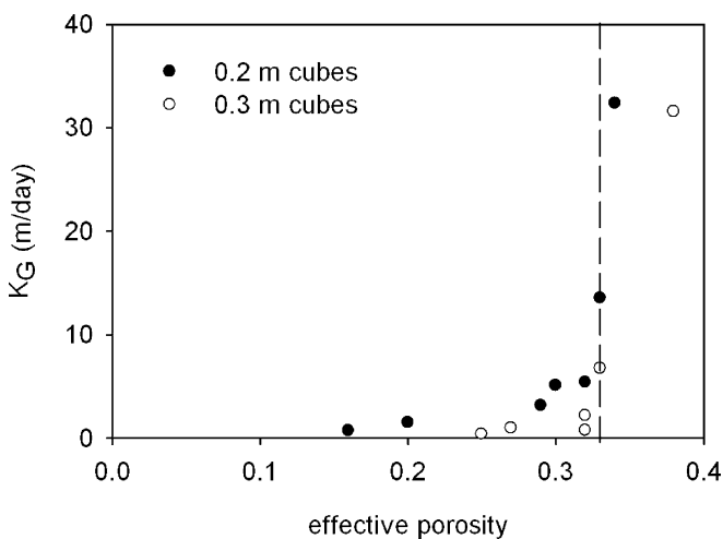
Fig. 8 Graph showing relationship between effective porosity and the geometric mean of the hydraulic conductivity ( K_G ) for the 0.2 and 0.3-m cubes. Dashed vertical line indicates effective porosity value (0.33) at which large changes in hydraulic conductivity were observed
