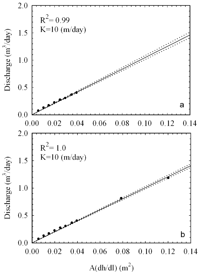
Fig. 7 Hydraulic conductivity results conducted on the vertical axis of 0.2-m cube No. 7 for hydraulic heads ranging from a 0.025 to 0.2 m and b 0.025 to 0.6 m. On both plots, the solid line represents the linear regression line through the data while the dotted line is the 95% confidence interval about the line. The slope of the best fit line ( K ) and R^2 for both plots is provided
