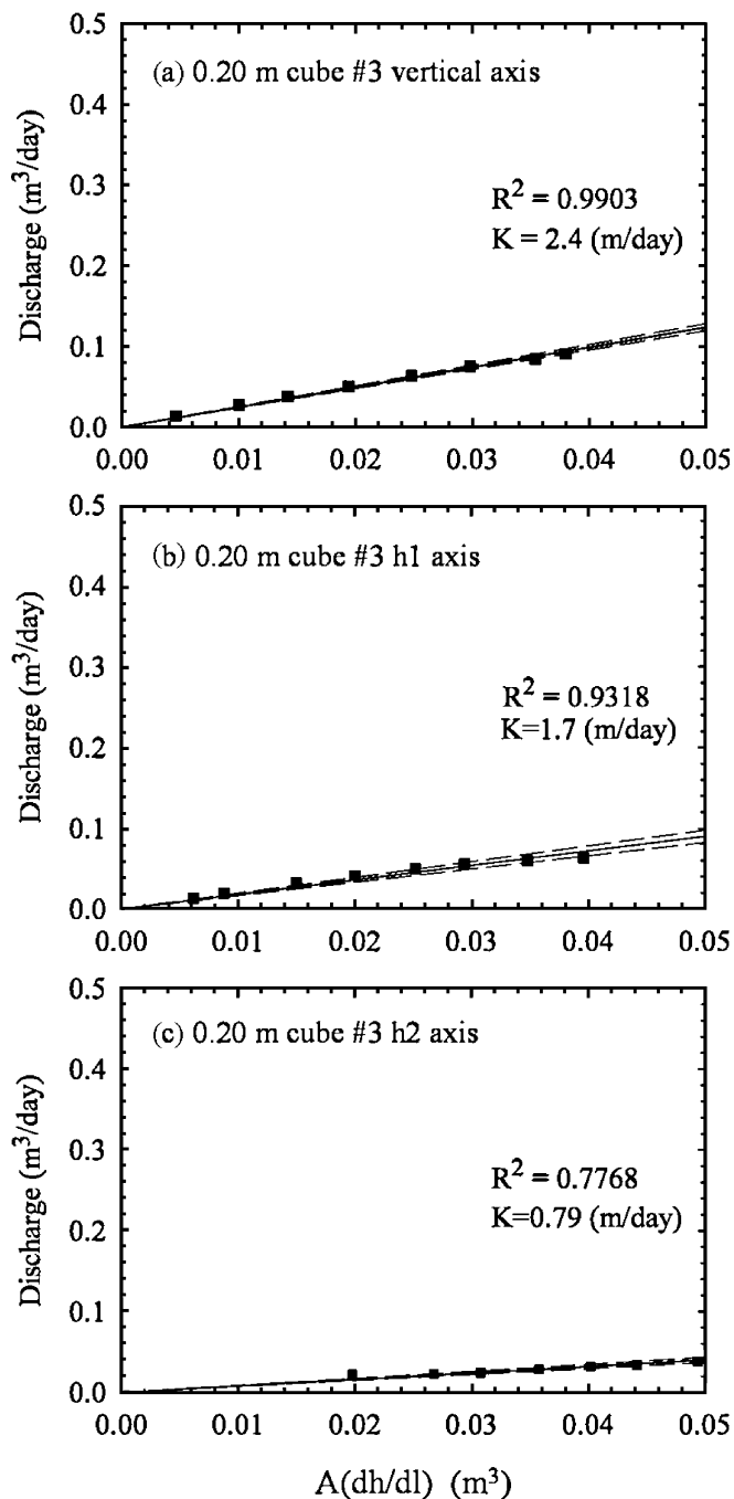
Fig. 5 Results of permeameter testing of three axes a vertical; b h1 and c h2 of the 0.2-m cube No. 3, demonstrating linearity between discharge and hydraulic gradient. The hydraulic conductivity was estimated as the slope of the linear regression line through the data
