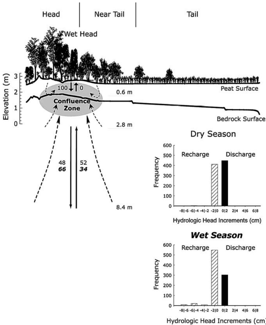
FIGURE 7. Hydrologic movements under Island 3A53 for dry (November–April) and wet (May–October) seasons (data collected August 2003 to June 2008 unless otherwise noted). Arrows indicate the percentage of time that water was discharging or recharging at designated depths (data at 0.6 m collected from 2007 and 2008). Bold, italicized numbers indicate wet season. Dotted arrows represent water movement from tree transpiration. Tree transpiration and the confluence of recharge and discharge create a chemical mixing zone of higher ionic concentrations and salinity that is most strongly present during the dry season. Histograms depict magnitude of hydraulic head in groundwater movement between 2.8 and 8.4 m deep. The x -axis values are 2 cm increments of head difference; the y -axis is the daily frequency of each increment. Surface and bedrock lines are from D. Mason (Indiana Dunes National Park, unpublished data).
