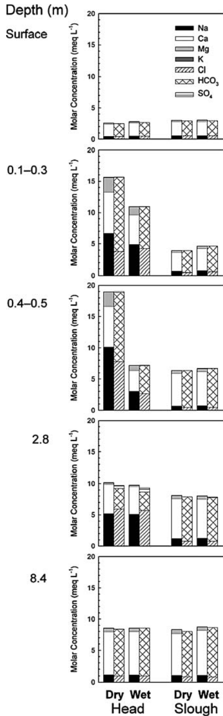
FIGURE 8. Mean ionic composition of water from wells located on the head of Island 3AS3 and surrounding marsh at various depths during dry (November–April) and wet (May–October) seasons. Data collected between 1999 and 2005.
