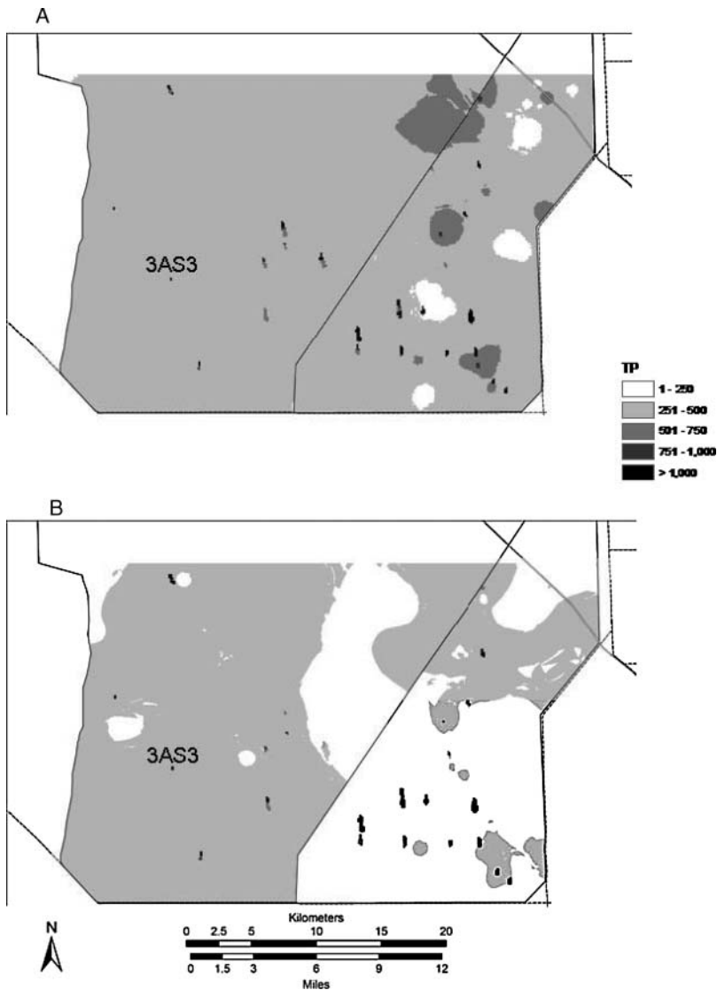
FIGURE 2. Spatial distribution of soil total phosphorus concentrations ( \text{mg kg}^{-1} ) in southern WCA-3A and WCA-3B. (A) Total soil phosphorus at 0–10 cm. (B) Total soil phosphorus at 10–20 cm deep. Only islands in which soil TP were measured are shown on these figures. There are many other tree islands in the areas depicted.
