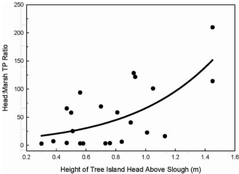
FIGURE 3. Relationship of height of tree island head above surrounding marsh and the ratio of island head to marsh total soil phosphorus levels (0–20 cm deep) for 31 islands located in WCA-3A and WCA-3B. For fitted line, r^2 = .44 , p = .004 .
