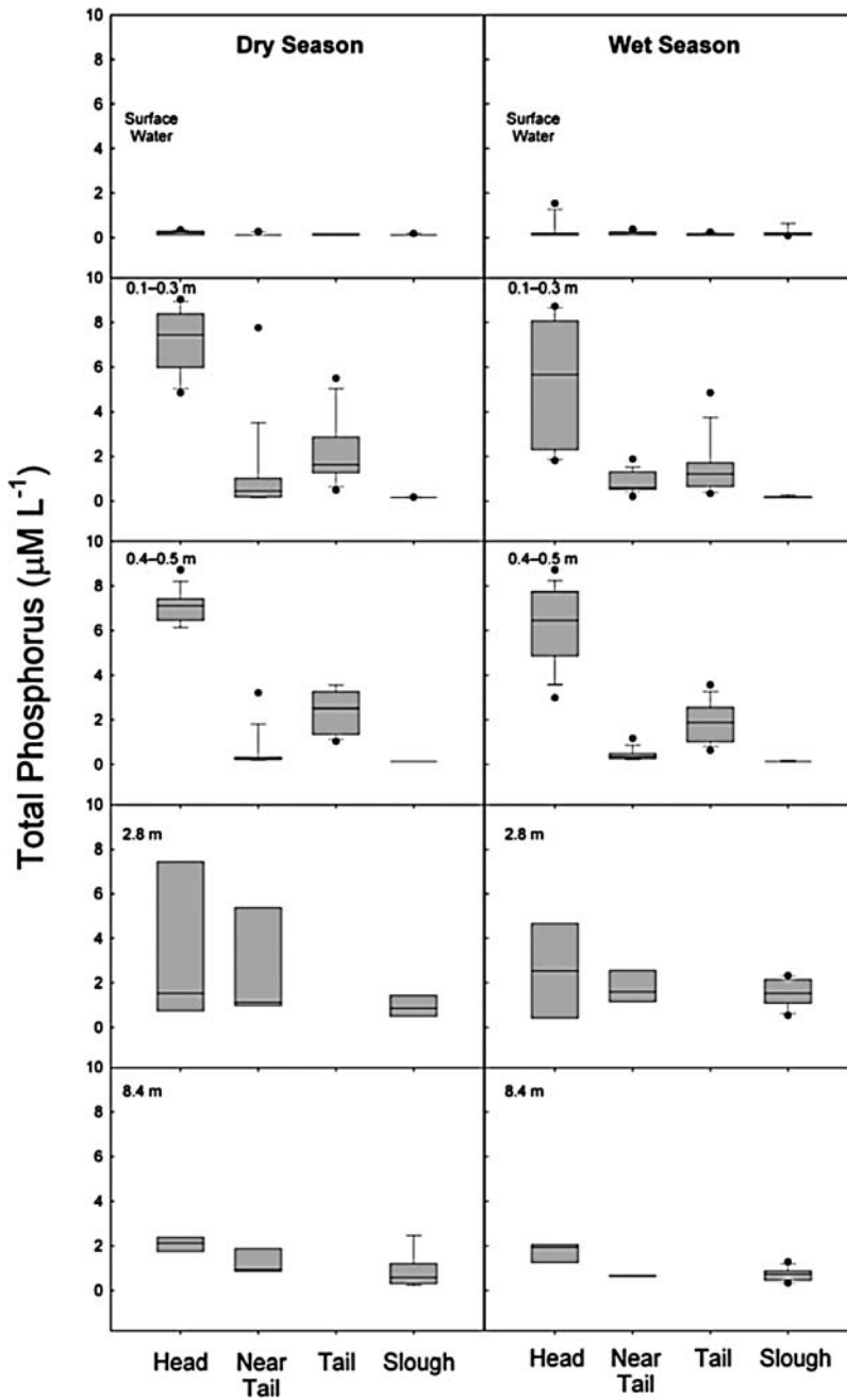
FIGURE 9. Total phosphorus in wells located on Island 3AS3 head, near tail, tail, and surrounding slough at various depths during dry (November–April) and wet (May–October) seasons. Data collected between 1999 and 2005.
