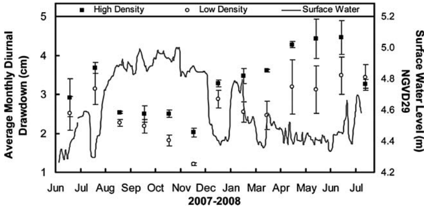
FIGURE 6. Average monthly diurnal drawdown from created tree islands at the Loxahatchee Impoundment Landscape Assessment facility. Two diurnal signatures are shown: one from a portion of the island with trees planted in high density (1 m spacing) and the second from a portion of the island planted with trees at low density (3 m spacing). Trees were between 4 and 5 years old. Surface water level during the data collection period is also shown.
