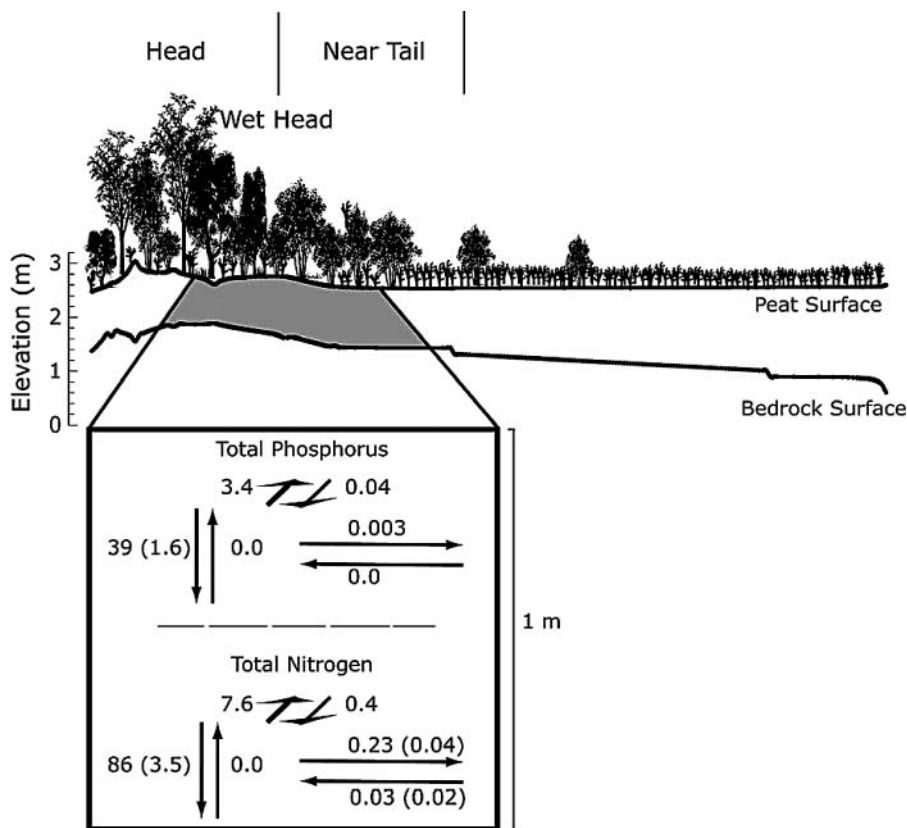
FIGURE 10. Dry season infiltration and lateral nutrient fluxes in the root zone on wet head and near tail of Island 3AS3. Total phosphorus and nitrogen fluxes ( \text{mg m}^{-2} \text{d}^{-1} ) between 0.3 and 0.6 m deep. Lateral fluxes are the sums of averaged values across a transect. Dry season data collected from March 2 to 21, 2007.
