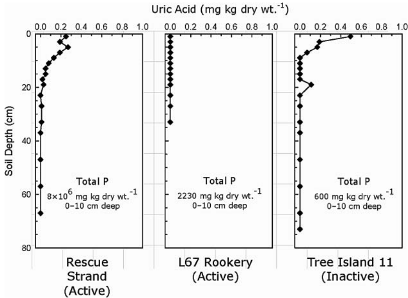
FIGURE 4. Distribution of uric acid with soil depth on two islands with active bird rookeries and an island with an inactive bird rookery.
