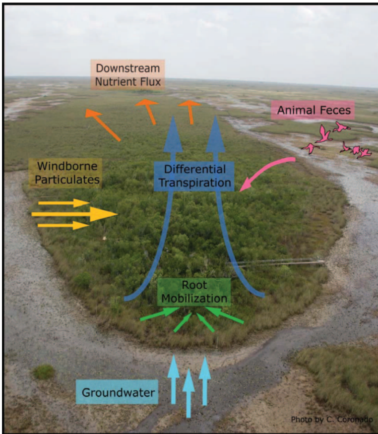
FIGURE 1. The Focused Nutrient Redistribution hypothesis proposes that forested islands capture and focus nutrients on the Everglades landscape through transpiration, attraction of animals, capture of aeolian deposits, groundwater upwelling, and alteration of the rhizosphere environment. Downstream nutrient fluxes enhance plant growth, increasing organic matter deposition and further tree growth, causing the island to expand. The photograph is of intensively studied Island 3AS3, located in the southwest WCA-3A. Note boardwalks on island head and near tail. (This figure is available in color online.)
