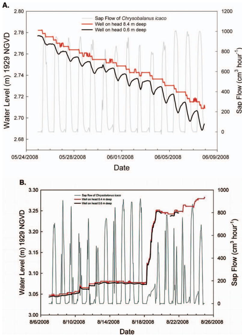
FIGURE 5. Diurnal well water levels and sap flow from the head of Island 3AS3 in dry and wet seasons. Daily sap flow velocities for Chrysobalanus icaco are also shown. (A) Dry season: Diurnal water level in root zone (0.6 m deep), shallow (2.8 m deep), and deep (8.4 m deep) wells. Data collected from 25 May to 8 June, 2008. (B) Wet season: Diurnal water level in root zone (0.6 m deep), shallow (2.8 m deep), and deep (8.4 m deep) wells. Data collected August 6–26, 2008. (This figure is available in color online.)
